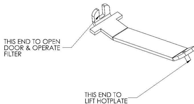
Figure 4 Operating Tool and Glove
