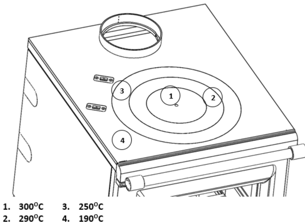
Figure 9 Approx. Working Temperatures 30 Mins. After Refueling
